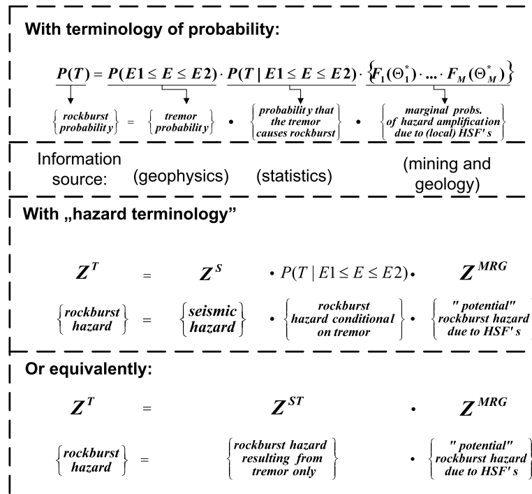
Fig. 1. Basic decomposition forms of rockburst hazard estimator, Z^T HSF – hazard shaping factor
